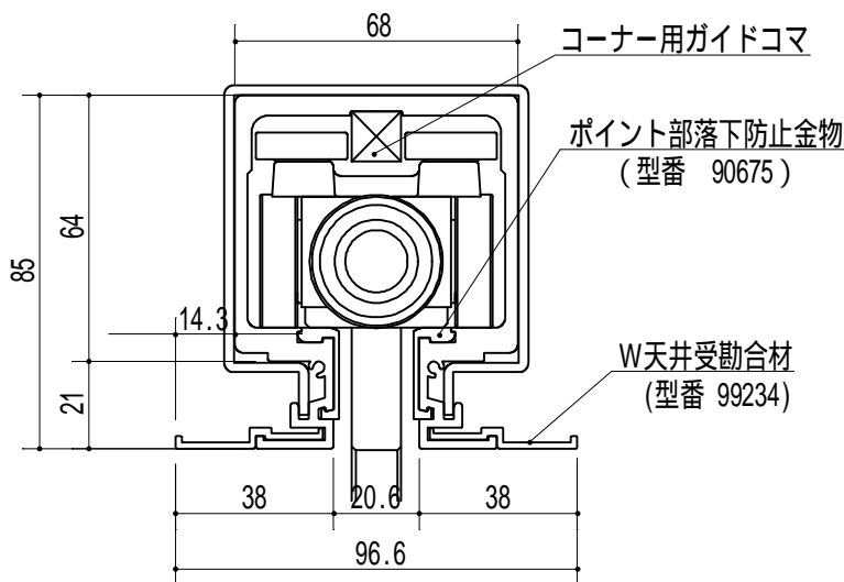
W天井受働合材組込型断面図 (1/2)
